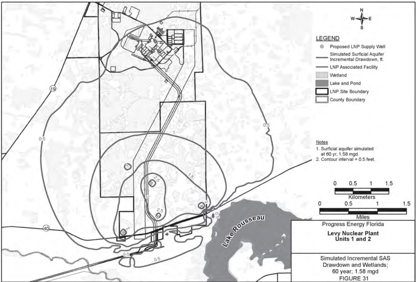
Figure 5-1. Simulated Incremental Surficial Aquifer System (SAS) Drawdown Associated with LNP Operations (PEF 2010a)
