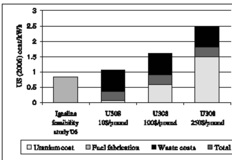
Graph: Nuclear Fuel Cost Comparison per kWh electricity
